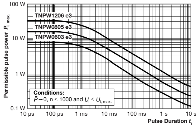
Maximum pulse load, single pulse; applicable if \bar{P} \rightarrow 0 and n \leq 1000 and \hat{U} \leq \hat{U}_{max} ; for permissible resistance change \pm (0.5 \% R + 0.05 \Omega)
