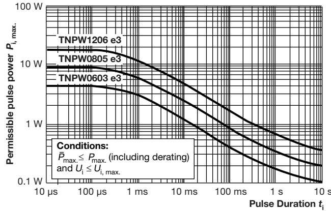
Maximum pulse load, continuous pulse; applicable if \bar{P} \leq P(\vartheta_{amb}) and \hat{U} \leq \hat{U}_{max} ; for permissible resistance change \pm (0.5 \% R + 0.05 \Omega)
