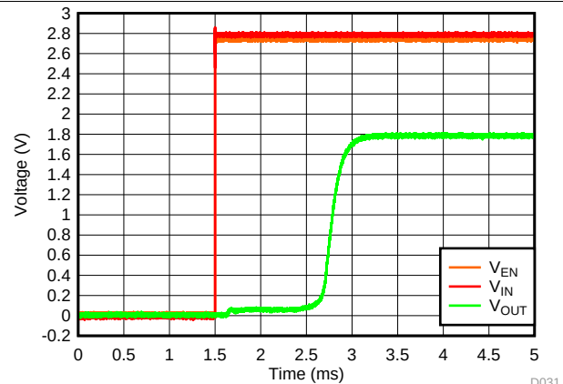
Figure 32. Startup With V_{EN} = V_{IN}
