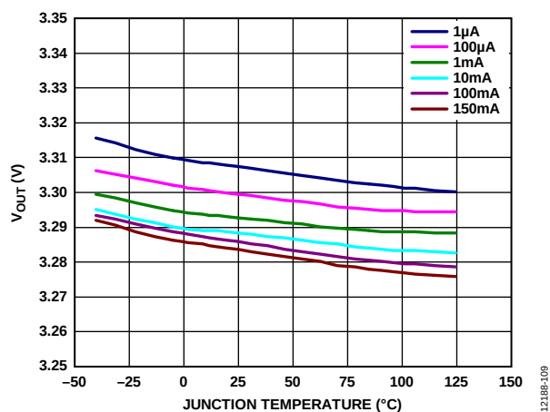
Figure 9. Output Voltage ( V_{OUT} ) vs. Junction Temperature
