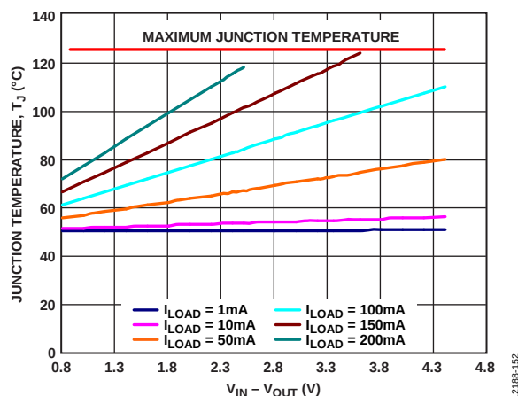
Figure 54. 100 mm 2 of PCB Copper, LFCSP, T_A = 50^{\circ}\text{C}
