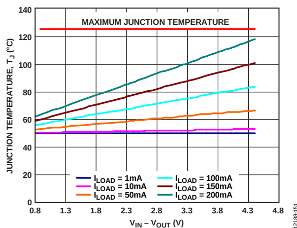
Figure 53. 500 mm 2 of PCB Copper, LFCSP, T_A = 50^{\circ}\text{C}
