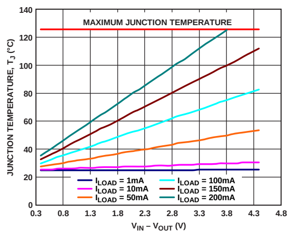
Figure 47. 500 mm 2 of PCB Copper, TSOT, T_A = 25^\circ\text{C}
