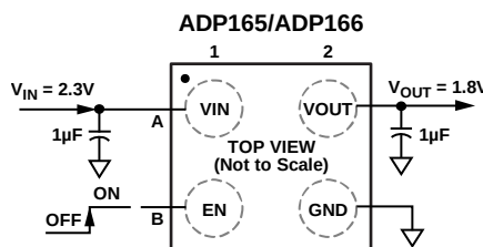
Figure 3. 4-Ball WLCSP ADP165/ADP166 with Fixed Output Voltage, 1.8 V
