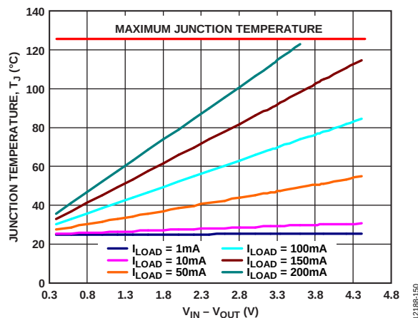
Figure 52. 100 mm 2 of PCB Copper, LFCSP, T_A = 25^{\circ}\text{C}
