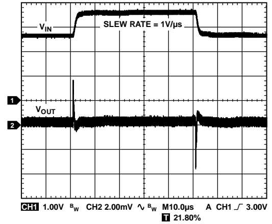
Figure 38. Line Transient Response, 1V Input Step, I_{LOAD} = 1.2\text{ A} , V_{OUT} = 1.8\text{ V} , V_{IN} = 2.5\text{ V} , Channel 1 = V_{IN} , Channel 2 = V_{OUT}
