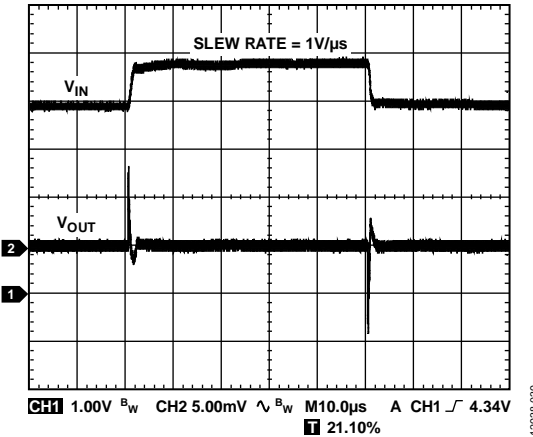
Figure 37. Line Transient Response, 1V Input Step, I_{LOAD} = 1.2\text{ A} , V_{OUT} = 3.3\text{ V} , V_{IN} = 3.8\text{ V} , Channel 1 = V_{IN} , Channel 2 = V_{OUT}
