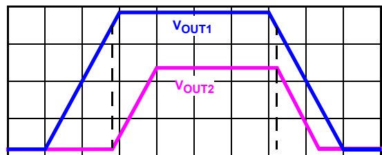
FIGURE 61. OUTPUT SEQUENCING
