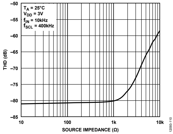
Figure 30. THD vs. Source Impedance
