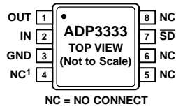
Figure 3. Pin Configuration
