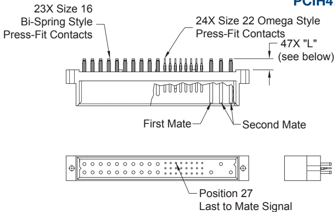
CONNECTOR DIMENSIONS
