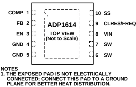
Figure 3. Pin Configuration
