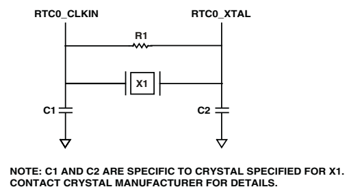
Figure 6. External Components for RTC
