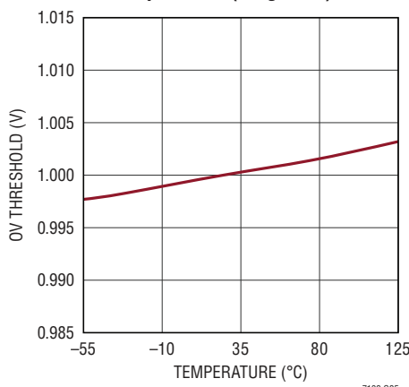
V OUT Overvoltage Threshold vs Temperature (Target 1V)
