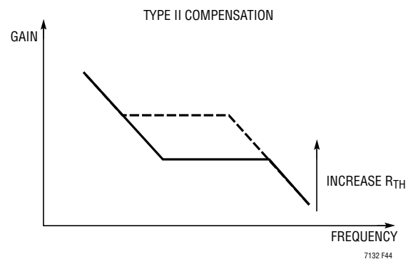
Figure 43. R_{TH} Adjust
