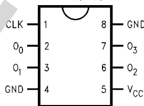
Pin Assignment SOIC (MO)
