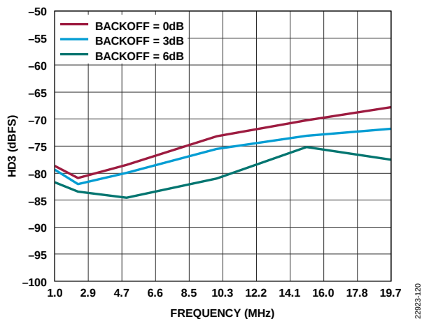
Figure 24. ADC HD3 vs. Frequency at Various Backoff Values and A_{IN} = -2 dB, 1 GSPS
