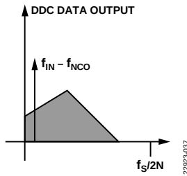
Figure 73. Output Spectrum of the DDC Output
