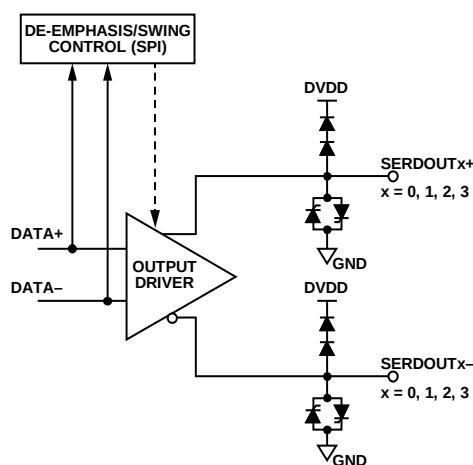
Figure 51. Digital Outputs
