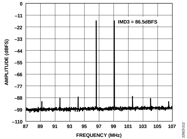
Figure 46. Two-Tone FFT, Backoff = 6, f_{IN1} = 96.6 MHz, f_{IN2} = 99 MHz, A_{IN1} and A_{IN2} = -16 dBFS, 2 GSFS
