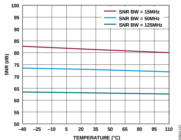
Figure 31. ADC SNR vs. Junction Temperature, 2 GSPS
