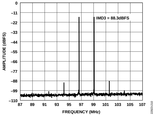
Figure 44. Two-Tone FFT, Backoff = 0, f_{IN1} = 96.6 MHz, f_{IN2} = 99 MHz, A_{IN1} and A_{IN2} = -16 dBFS, 2 GSFS
