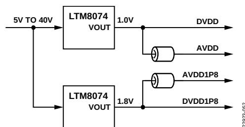
Figure 93. Simplified Power Solution for the AD9083
