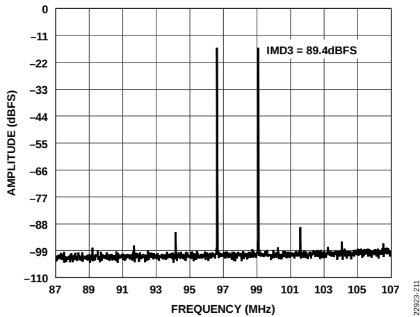
Figure 45. Two-Tone FFT, Backoff = 3, f_{IN1} = 96.6 MHz, f_{IN2} = 99 MHz, A_{IN1} and A_{IN2} = -16 dBFS, 2 GSFS
