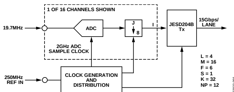
Figure 90. Wide Bandwidth Real Output Mode Block Diagram, See Table 1
