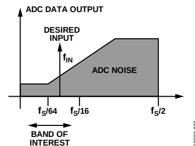
Figure 71. Spectrum of the Raw ADC Output
