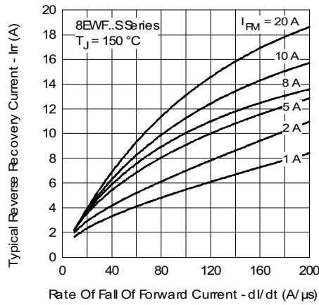
Fig. 13 - Recovery Current Characteristics, T J = 150 °C
