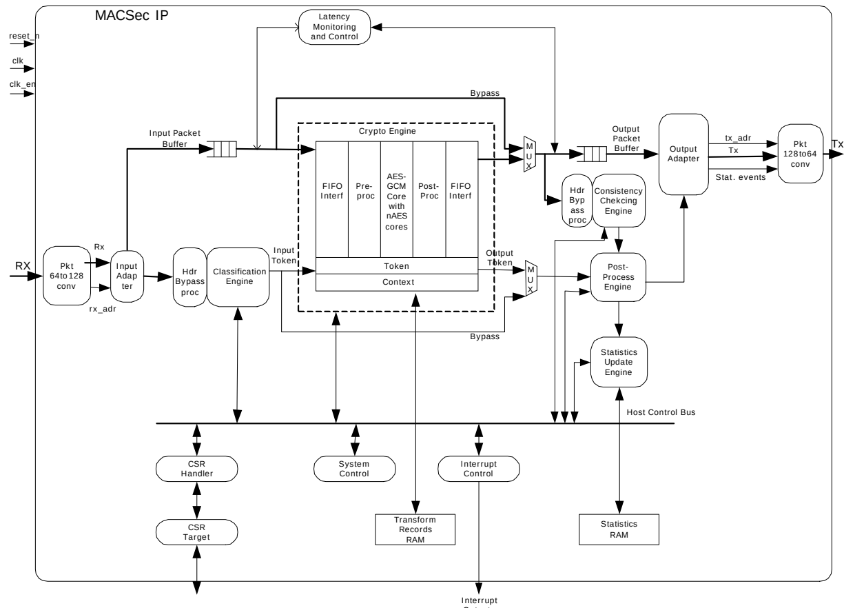
Figure 68 • MACsec Architecture
