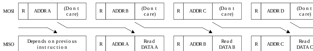
Figure 109 • SPI Multiple Register Reads
