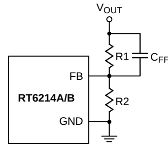
Figure 1. C_{\text{FF}} Capacitor Setting
