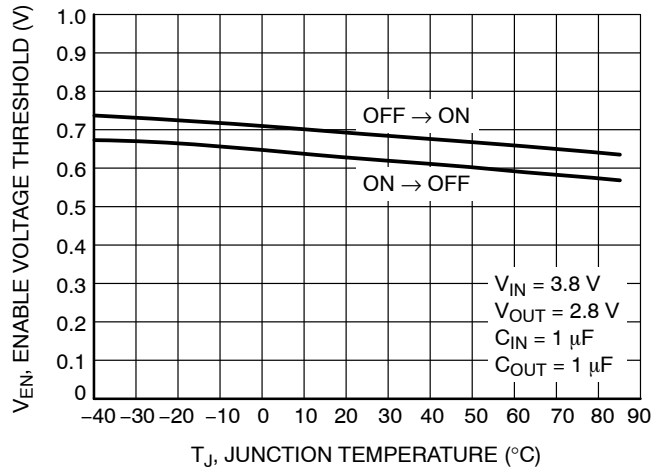
Figure 16. Enable Thresholds Voltage
