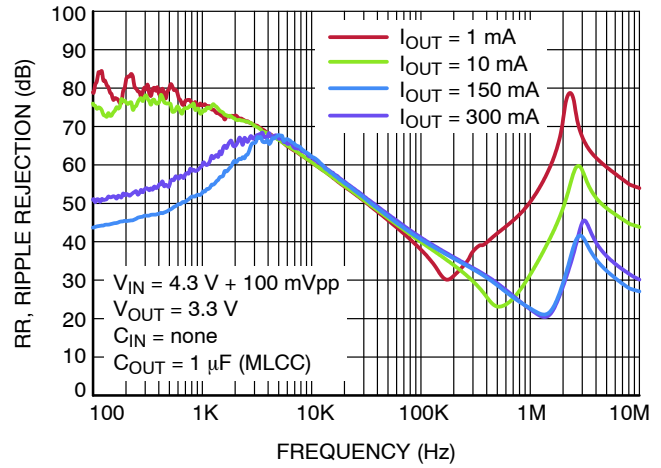
Figure 27. Power Supply Rejection Ratio, V_{OUT} = 3.3 V
