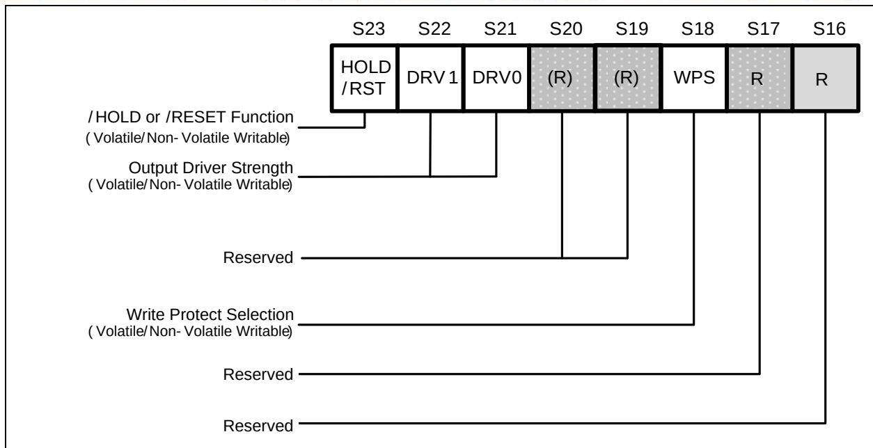
Figure 4c. Status Register-3
