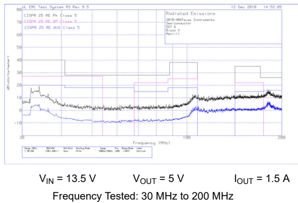
Figure 9-14. Radiated EMI Bicon Vertical vs. CISPR25 Limits
