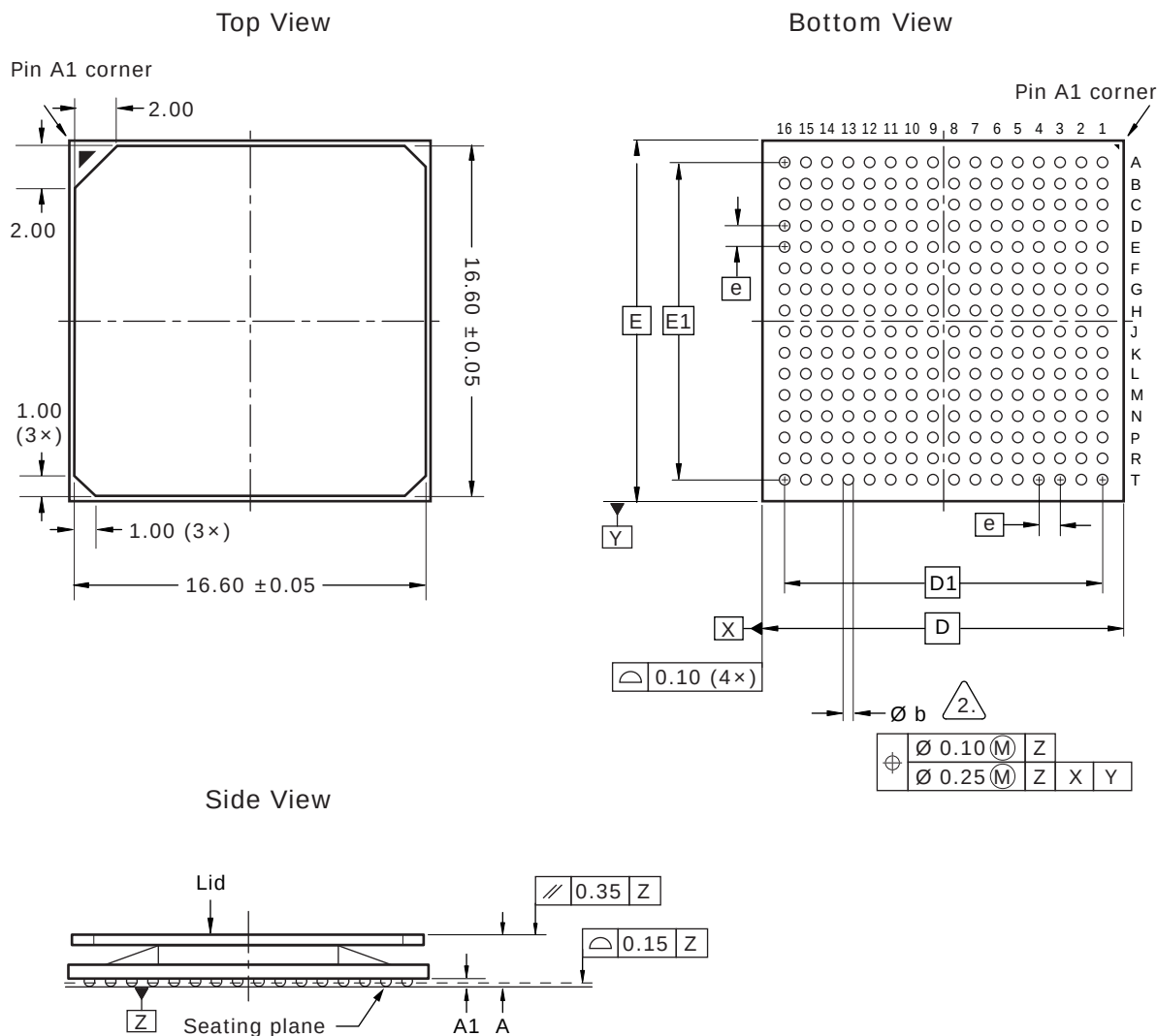
Figure 93 • VSC8257-01 Package
