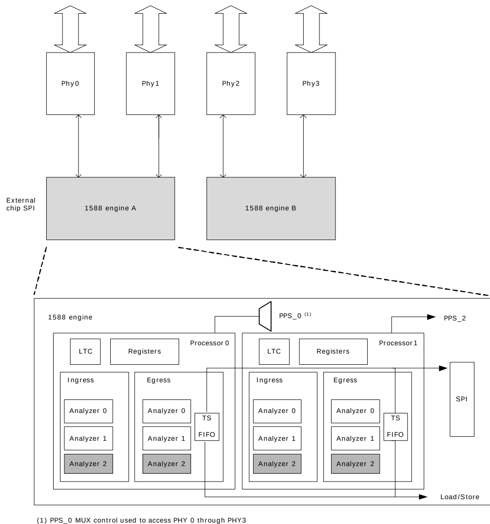
Figure 18 • IEEE 1588 Architecture
