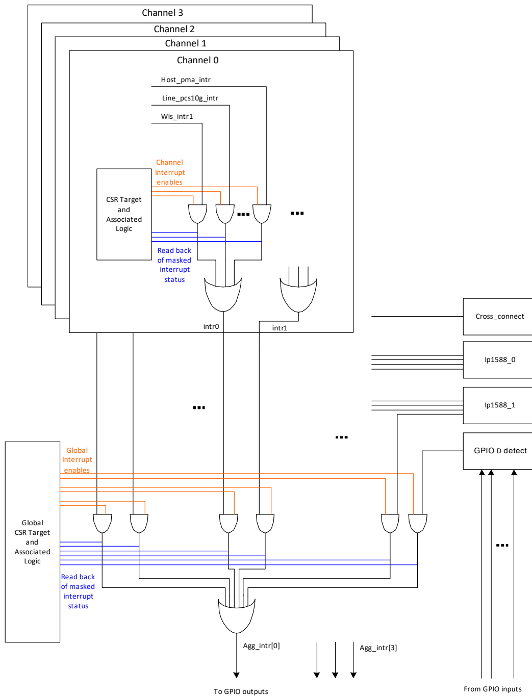
Figure 82 • Interrupt Scheme
