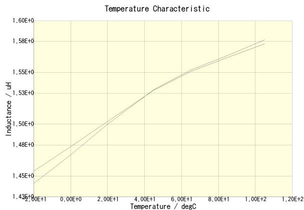
CLF7045T-1R5N-CA(DC = 0A)
