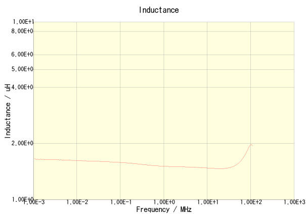
CLF7045T-1R5N-CA
