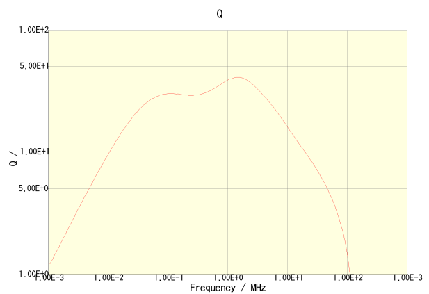
CLF7045T-1R5N-CA
