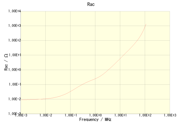
CLF7045T-1R5N-CA
