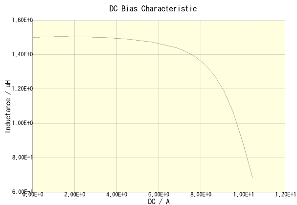
CLF7045T-1R5N-CA(Amb. Temp. = 20degc)
