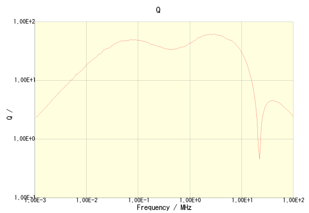
CLF7045T-220M-CA
