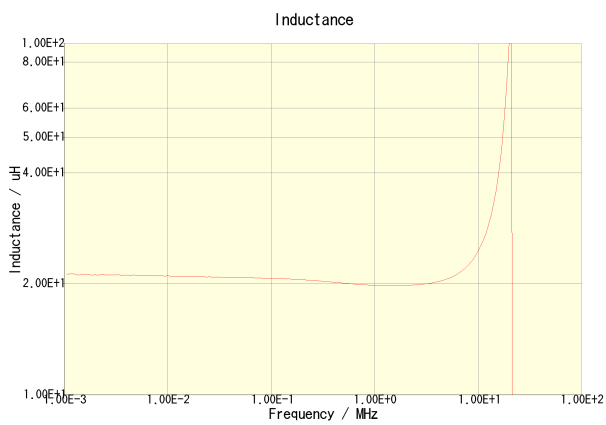
CLF7045T-220M-CA
