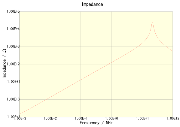
CLF7045T-220M-CA
