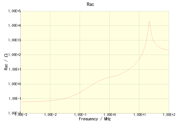
CLF7045T-220M-CA
