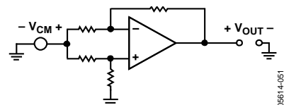
Figure 44. Common-Range Subtractor
