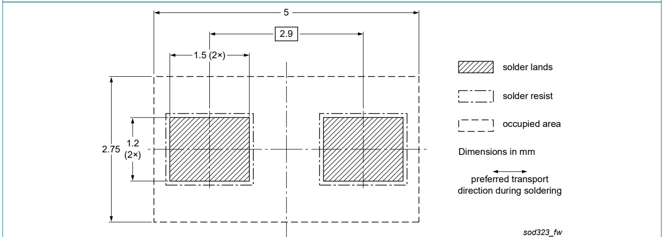
Fig. 10. Wave soldering footprint SOD323 (SC-76)
