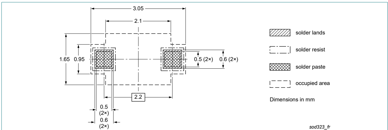
Fig. 9. Reflow soldering footprint SOD323 (SC-76)
