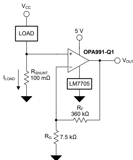
Figure 7-1. OPAx991-Q1 in a Low-Side, Current-Sensing Application
