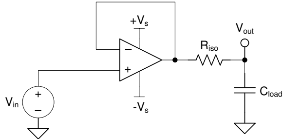
Figure 6-7. Extending Capacitive Load Drive With the OPAx991-Q1
