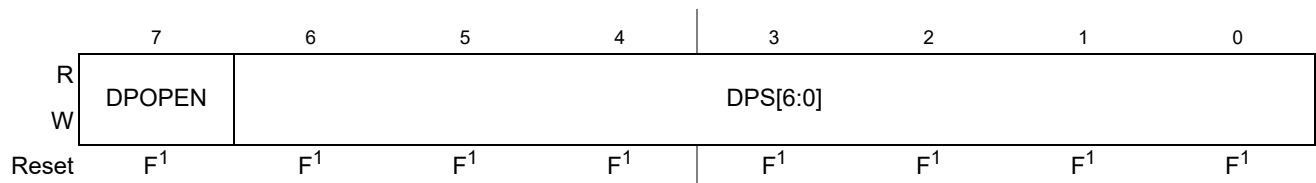
Figure 30-15. EEPROM Protection Register (EPROT)
