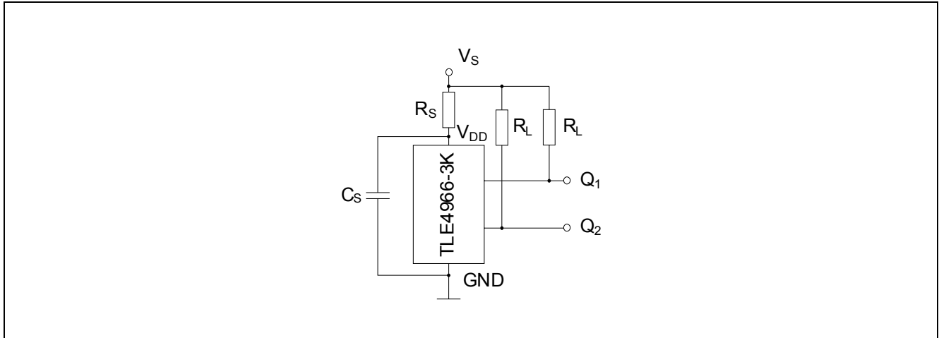
Figure 3 Application Circuit
