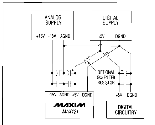
Figure 26. Power-Supply Grounding
