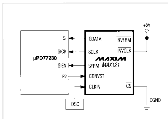
Figure 18. NEC \mu PD77230 Interface Circuit
