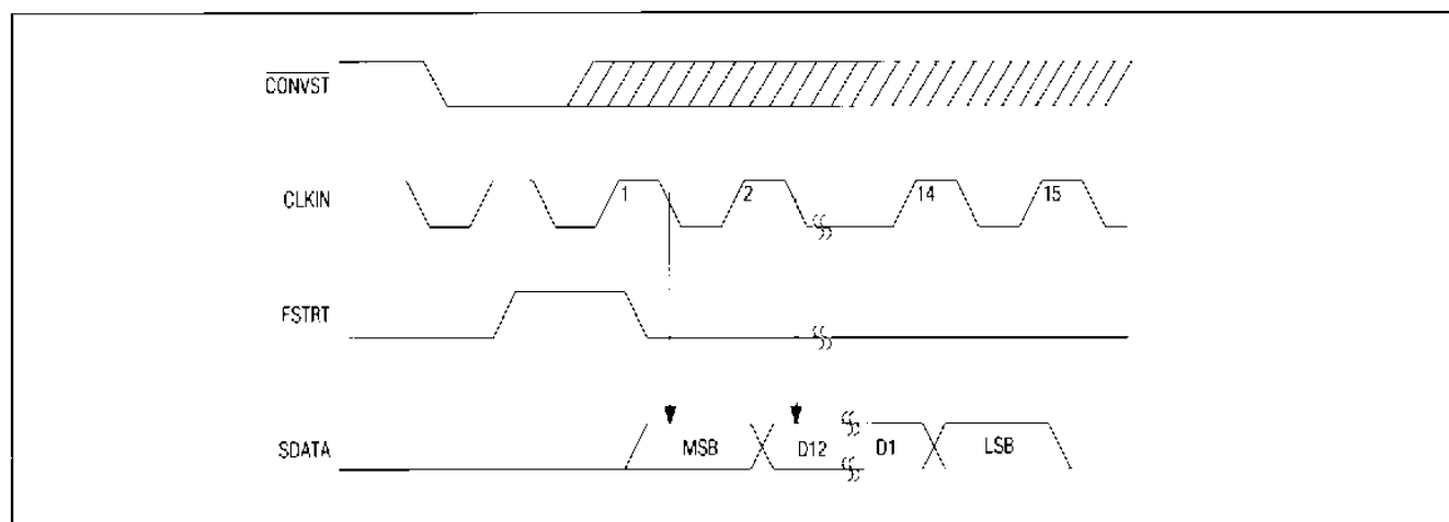
Figure 23. TMS320 Simple Serial-Interface Timing Diagram
