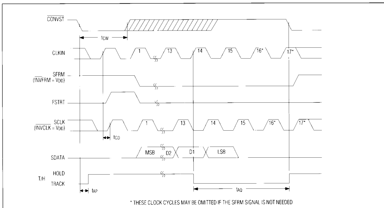
Figure 7. \overline{\text{CONVST}} Controls Conversion Starts (Mode 1)
