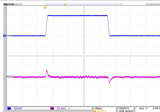
Figure 10-33. Line Transient Response
