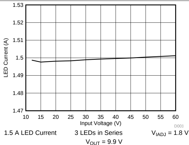
Figure 2. Line Regulation
