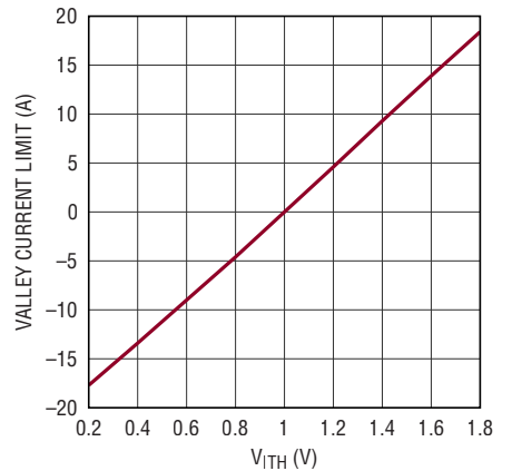
Valley Current Limit vs V_{ITH}
