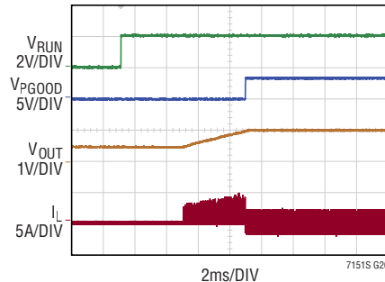
Start-Up with Pre-Biased Output, CCM
