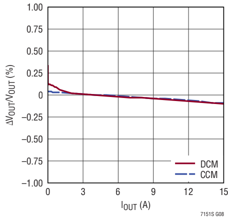
Load Regulation vs Load Current
