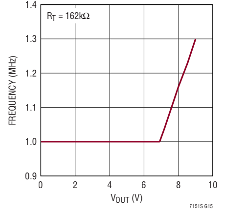
Switching Frequency vs V_{OUT}
