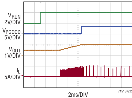
Start-Up with Pre-Biased Output, DCM
