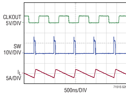
Continuous Conduction Mode Operation
