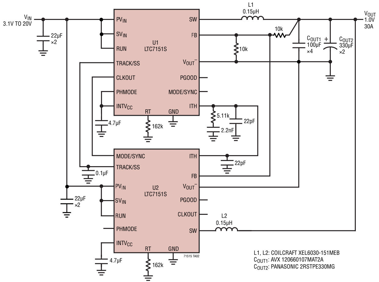
High Efficiency, Dual Phase 1.0V/30A Step-Down Supply
