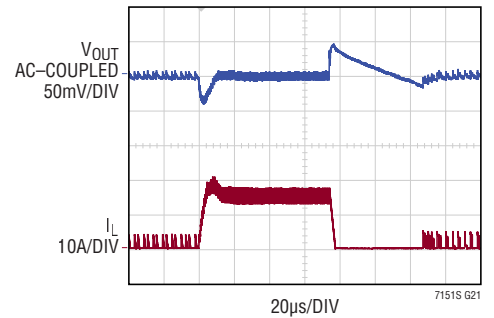
Transient Response, DCM
