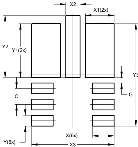
V-DFN3020-13/SWP (Type A1)
