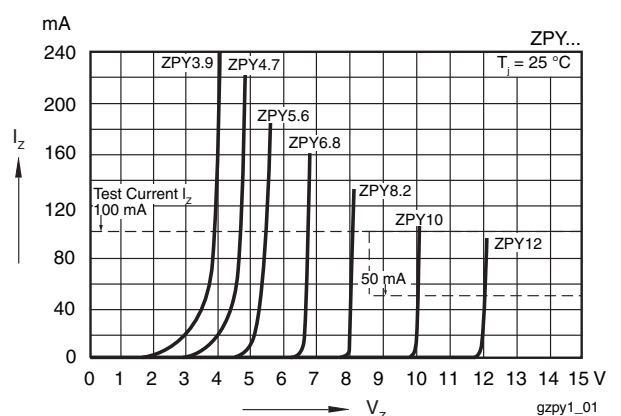
Fig. 6 - Breakdown Characteristics
