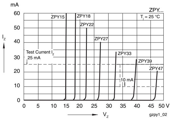
Fig. 7 - Breakdown Characteristics
