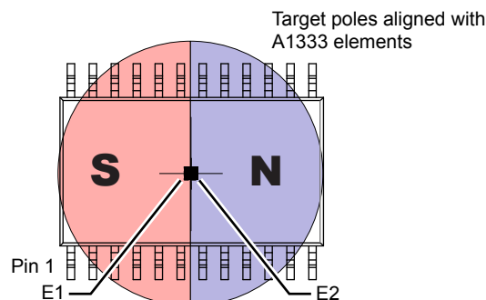
Figure 57: Orientation of Magnet Relative to Primary and Secondary Die
