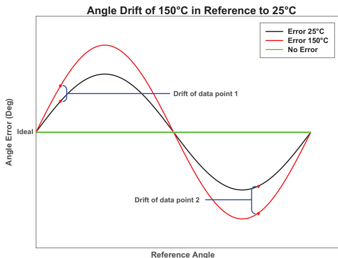
Figure 64: Angle Drift of 150°C in Reference to 25°C [1]
