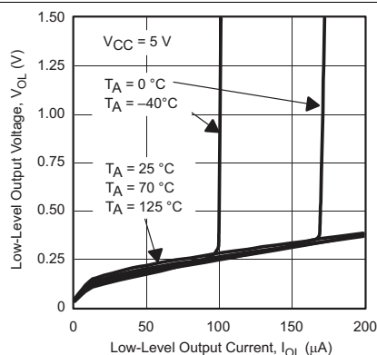
Figure 14. Low-Level Output Voltage vs Low-Level Output Current
