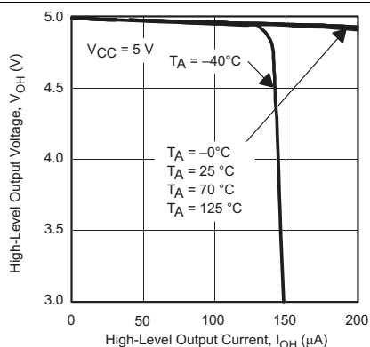
Figure 13. High-Level Output Voltage vs High-Level Output Current
