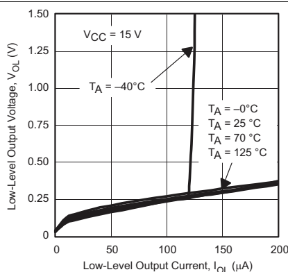
Figure 16. Low-Level Output Voltage vs Low-Level Output Current
