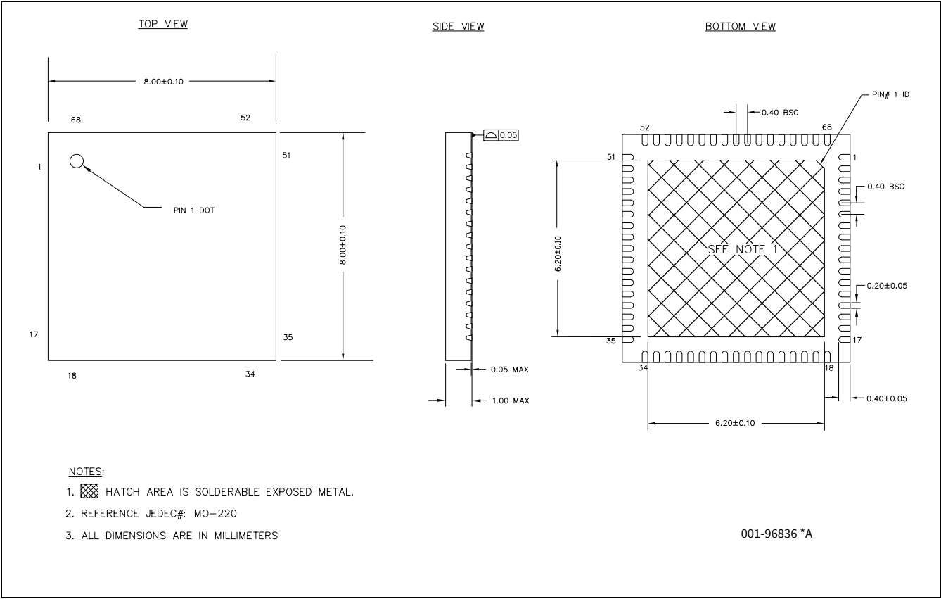
Figure 24 68 QFN 8 × 8 × 1 mm
