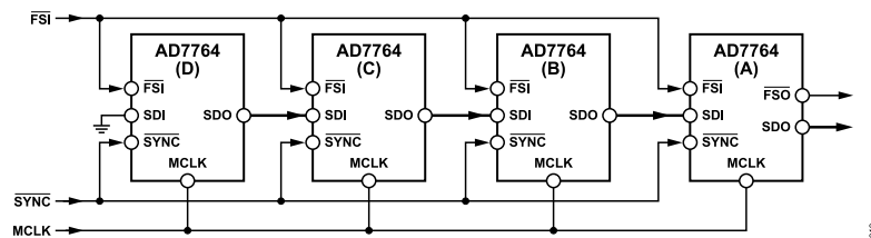
Figure 47. Daisy-Chaining Four Devices in Decimate 128x Mode Using a 40 MHz MCLK Signal
