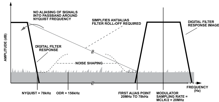
Figure 35. Antialias Example Using the AD7764 in Normal Mode, Decimate \times 128 Using MCLK/2 = f_{CLK} = 20 MHz
