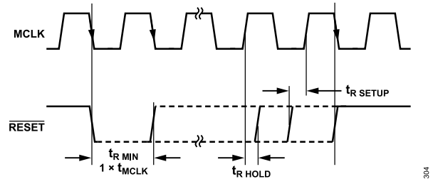
Figure 46. \overline{\text{RESET}} Timing Synchronous to MCLK
