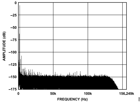
Figure 6. Normal Power Mode, FFT, 1 kHz, -0.5\text{ dB} Input Tone, 64x Decimation Rate
