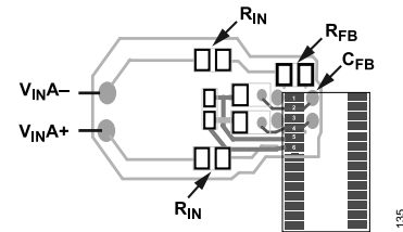
Figure 55. Typical Layout Structure for Components Surrounding the Differential Amplifier
