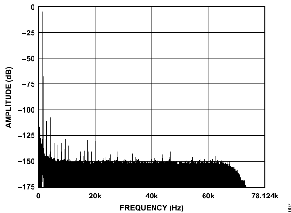
Figure 7. Normal Power Mode, FFT, 1 kHz, -0.5\text{ dB} Input Tone, 128x Decimation Rate
