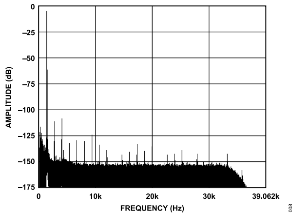
Figure 8. Normal Power Mode, FFT, 1 kHz, -0.5\text{ dB} Input Tone, 256x Decimation Rate
