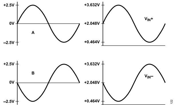
Figure 38. Differential Amplifier Signal Conditioning
