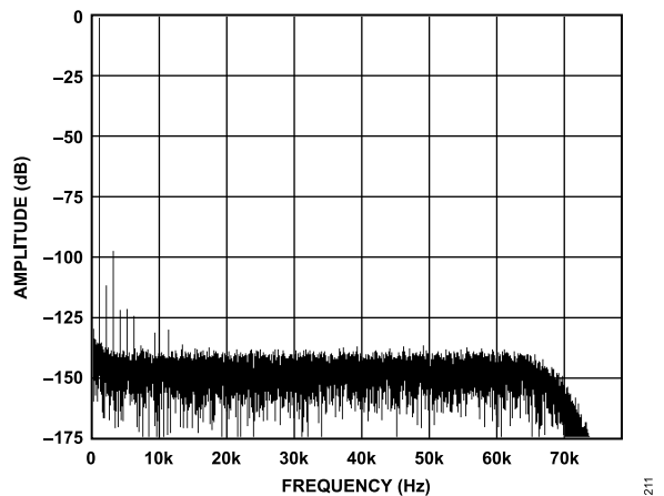
Figure 10. Low Power Mode, FFT, 1 kHz, -0.5\text{ dB} Input Tone, 128x Decimation Rate
