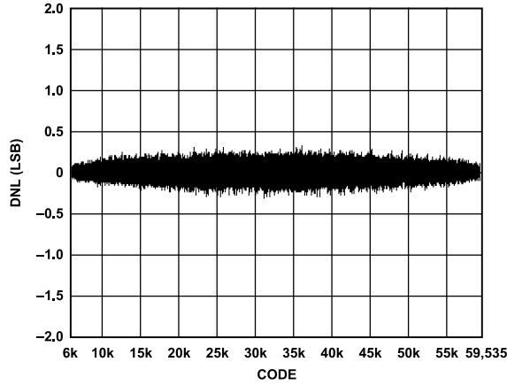
Figure 24. DNL Plot
