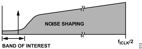
Figure 31. \Sigma - \Delta ADC, Noise Shaping
