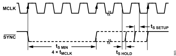
Figure 43. \overline{\text{SYNC}} Timing Relative to MCLK
