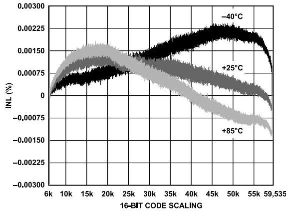
Figure 25. Normal Power Mode INL
