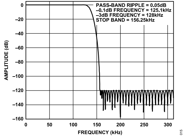
Figure 33. Filter Frequency Response (312.5 kHz ODR)
