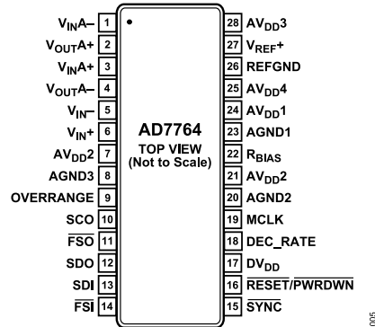
Figure 5. Pin Configuration
