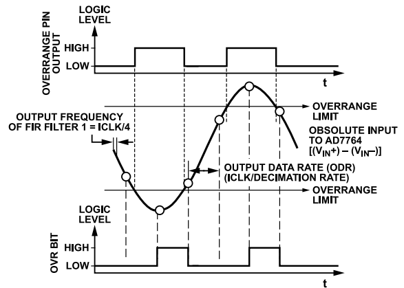
Figure 44. OVERRANGE Pin and OVR Bit vs. Absolute Voltage Applied to the Modulator
