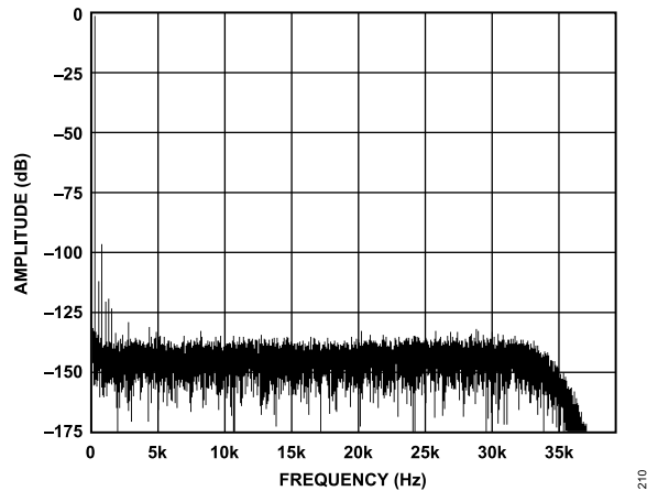
Figure 11. Low Power Mode, FFT, 1 kHz, -0.5\text{ dB} Input Tone, 256x Decimation Rate
