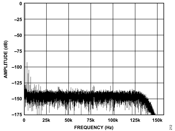
Figure 9. Low Power Mode, FFT, 1 kHz, -0.5\text{ dB} Input Tone, 64x Decimation Rate
