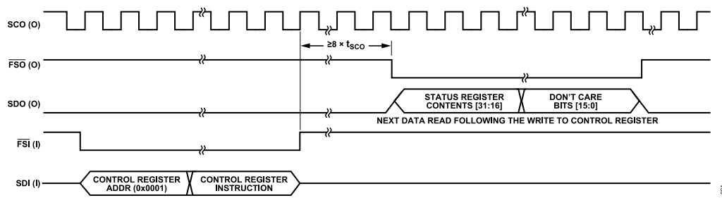
Figure 4. Status Register Read Cycle Timing Diagram
