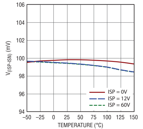
V_{(ISP-ISN)} Regulation vs Temperature
