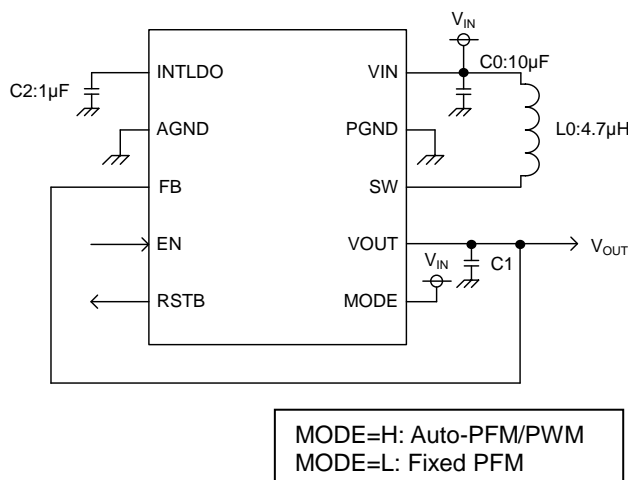
Figure 1. Application Circuit
