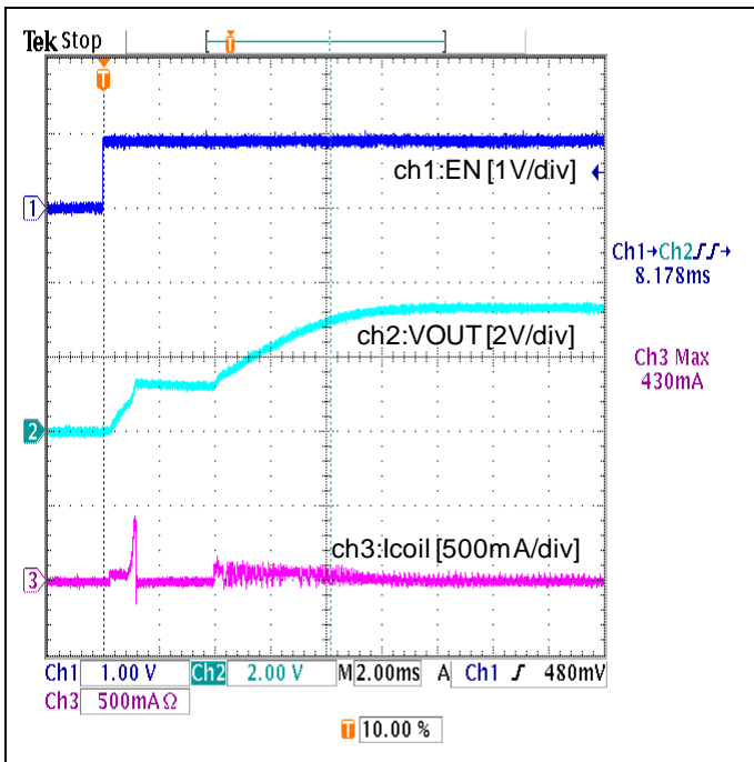
Figure 23. Start-up Waveform (VIN=0.9V, 3.3kΩ resistive load, MODE=H: Auto-PFM/PWM)
