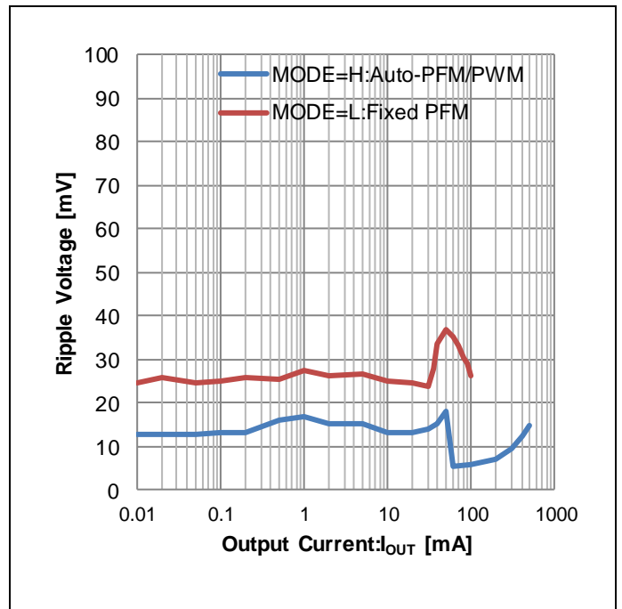
Figure 16. Ripple Voltage vs Output Current (VIN=2.4V)
