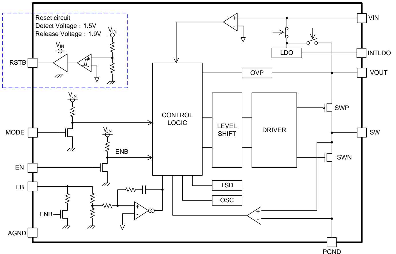
Figure 4. Circuit Block
