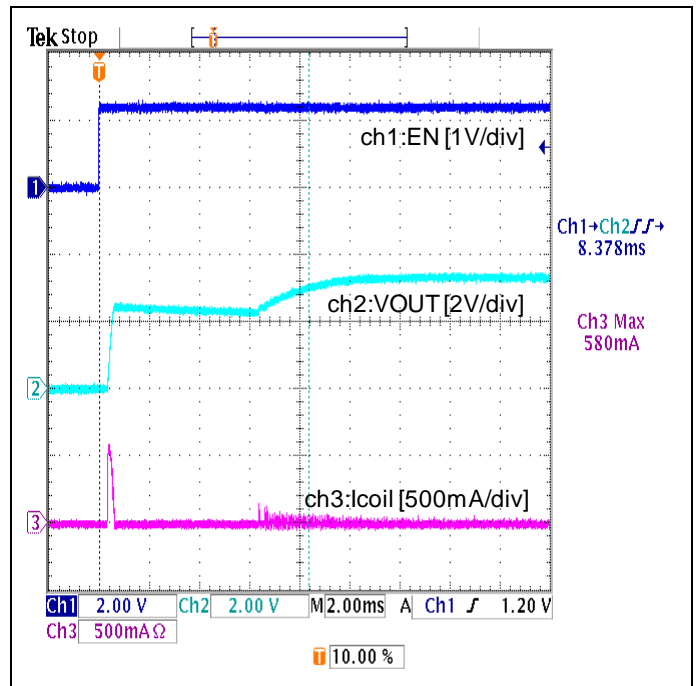
Figure 24. Start-up Waveform (VIN=2.4V, 3.3kΩ resistive load, MODE=H: Auto-PFM/PWM)
