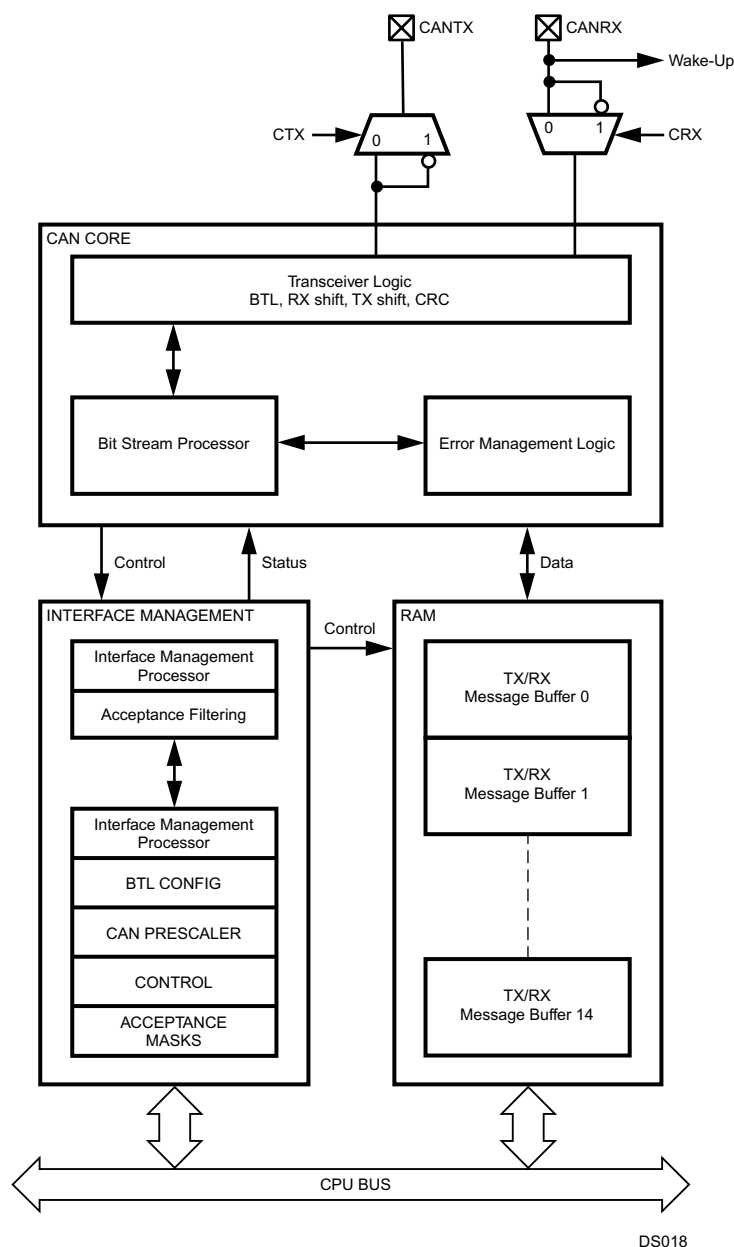
Figure 19-1. CAN Block Diagram
