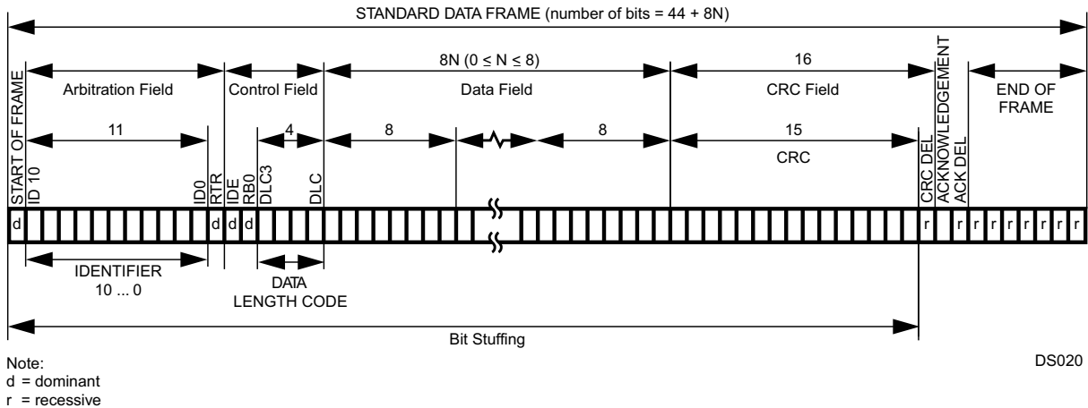
Figure 19-3. Standard Data Frame
