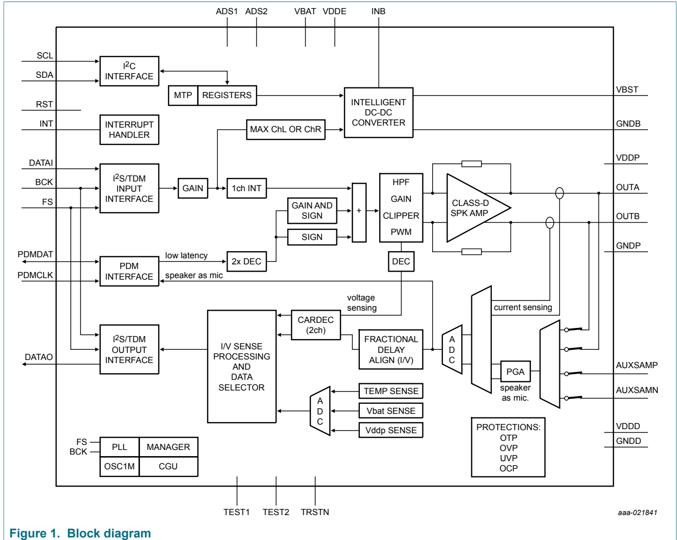
Figure 1. Block diagram
