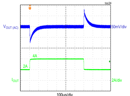
CONDITIONS: 3.3V OUTPUT, PWM/PFM/DCM MODE
