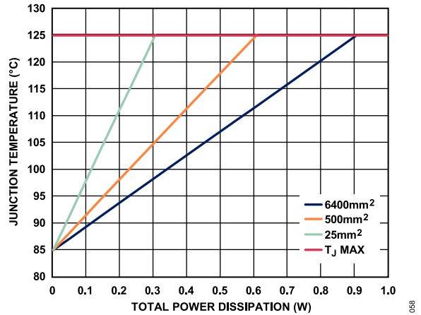
Figure 55. Junction Temperature vs. Total Power Dissipation for the 10-Lead LFCSP, T_A = 85^\circ\text{C}
