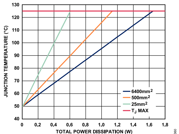
Figure 57. Junction Temperature vs. Total Power Dissipation for the 8-Lead SOIC, T_A = 50^\circ\text{C}
