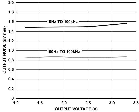
Figure 28. RMS Output Noise vs. Output Voltage
