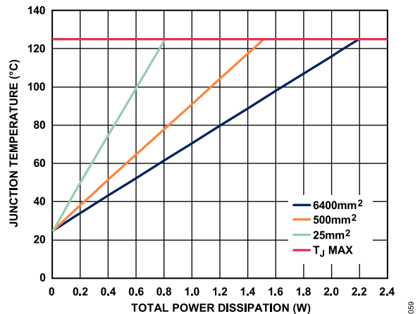
Figure 56. Junction Temperature vs. Total Power Dissipation for the 8-Lead SOIC, T_A = 25^\circ\text{C}
