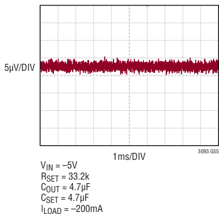
Output Noise (10Hz to 100kHz)
