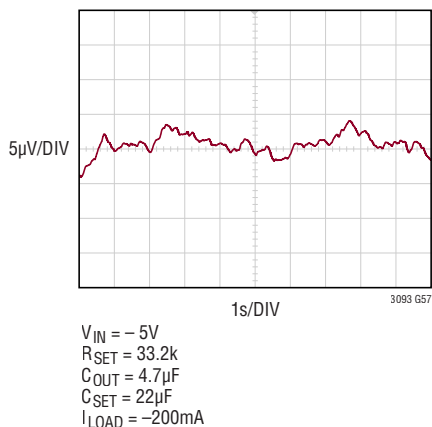
Output Voltage Noise (0.1Hz to 10Hz)
