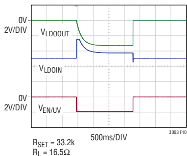
Figure 10. LT3093 EN/UV Pulse
