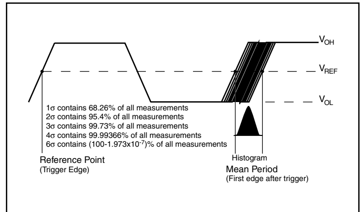
Period Jitter
