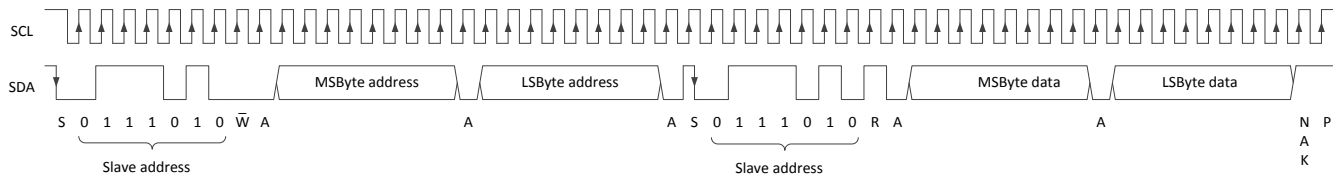
Figure 12: Addressed read
