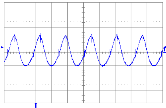
Fig. 1.2V.6: Output voltage ripple (20 mV/div.) at full rated load current into a resistive load with external capacitance 10 \mu\text{F} ceramic + 1 \mu\text{F} ceramic and V_{in} = 5\text{ V} for V_{out} = 1.2\text{ V} . Time scale: 2 \mu\text{s} /div.
