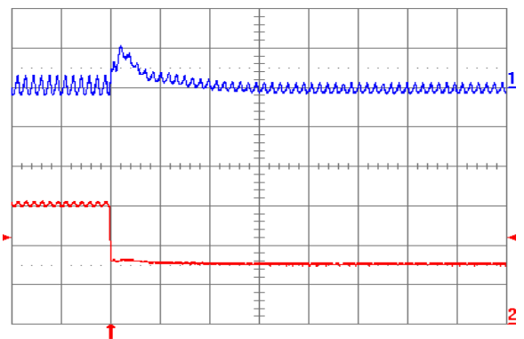
Fig. 1.2V.8: Output voltage response for V_{out} = 1.2\text{ V} to negative load current step change from 5 A to 2.5 A with slew rate of -5 A/ \mu\text{s} at V_{in} = 5\text{ V} . Top trace: output voltage (100 mV/div.); Bottom trace: load current (2 A/div.). C_o = 47\text{ }\mu\text{F} ceramic + 1 \mu\text{F} ceramic. Time scale: 20 \mu\text{s} /div.
