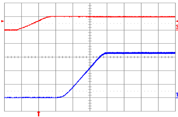
Fig. 3.3V.5: Turn-on transient for V_{out} = 3.3\text{ V} with application of V_{in} at full rated load current (resistive) and 47\text{ }\mu\text{F} external capacitance at V_{in} = 5\text{ V} . Top trace: V_{in} (5 V/div.); Bottom trace: output voltage (1V/div.); Time scale: 2 ms/div.
