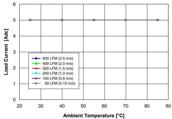
Fig. 2.5V.2: Available load current vs. ambient temperature and airflow rates for V_{out} = 2.5\text{ V} converter mounted horizontally with V_{in} = 5\text{ V} , air flowing from pin 5 to pin 1 and maximum MOSFET temperature \leq 120\text{ }^\circ\text{C} .
