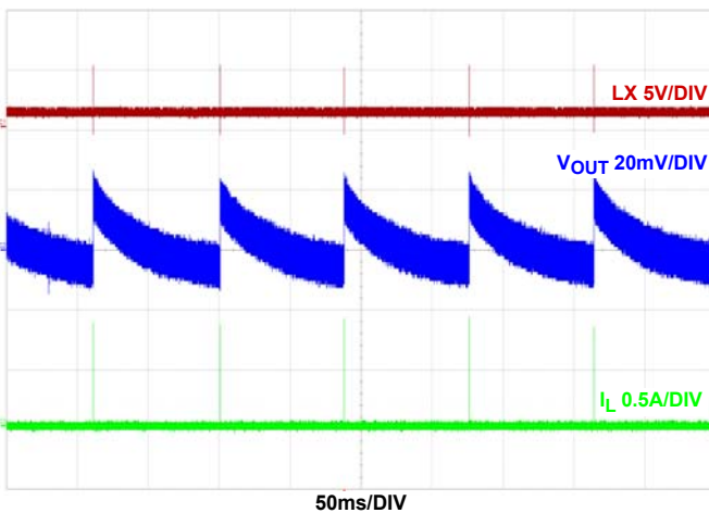
FIGURE 43. STEADY STATE AT NO LOAD F_{SW} = 2\text{MHz} , V_{IN} = 5\text{V} , MODE = PFM, T_A = +25^\circ\text{C}
