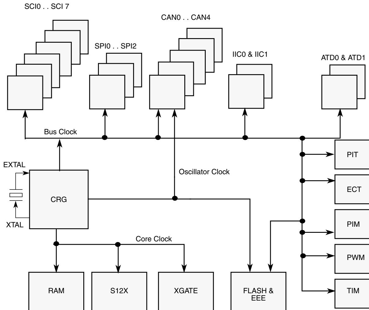
Figure 1-9. Clock Connections
