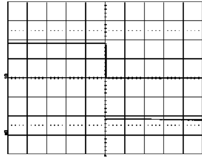
Shut-down enabled by disconnecting V_i at: T_{ref} = +25^\circ\text{C} , I_O = 6\text{ A} resistive load, V_i = 5.0\text{ V} . Top trace: output voltage (1.0 V/div.). Bottom trace: input voltage (5 V/div.). Time scale: 20.0 ms/div.
