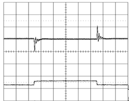
Output voltage response to load current step- change (3-6-3 A) at: T_{ref} = +25^\circ\text{C} , V_i = 5.0\text{ V} . Top trace: output voltage (100mV/div.). Bottom trace: load current (10 A/div.). Time scale: 0.1 ms/div.
