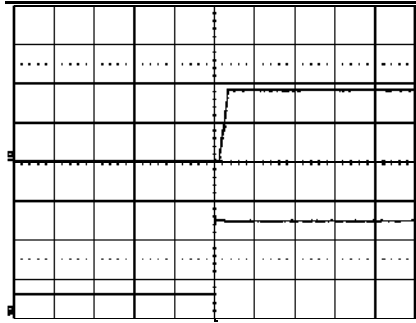
Start-up enabled by connecting V_i at: T_{ref} = +25^\circ\text{C} , I_O = 6\text{ A} resistive load, V_i = 5.0\text{ V} . Top trace: output voltage (1.0 V/div.). Bottom trace: input voltage (2 V/div.). Time scale: 20 ms/div.
