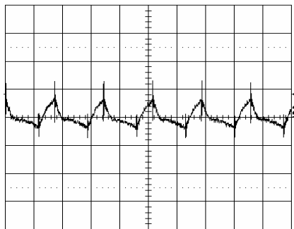
Output voltage ripple (20mV/div.) at: T_{ref} = +25^\circ\text{C} , I_O = 6\text{ A} resistive load, V_i = 5.0\text{ V} . Time scale: 1 \mu\text{s}/\text{div} . See the filter in the Output ripple and noise section (EMC Specification).
